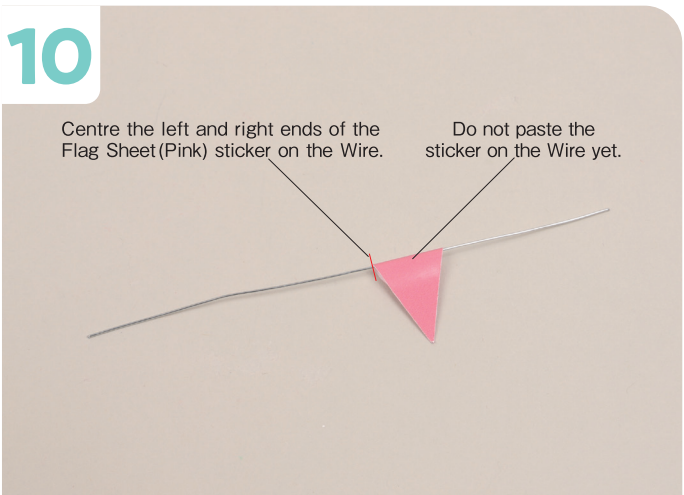
Adjust the position of the Flag Sheet (Pink) sticker so its left and right ends are centred on the Wire.
